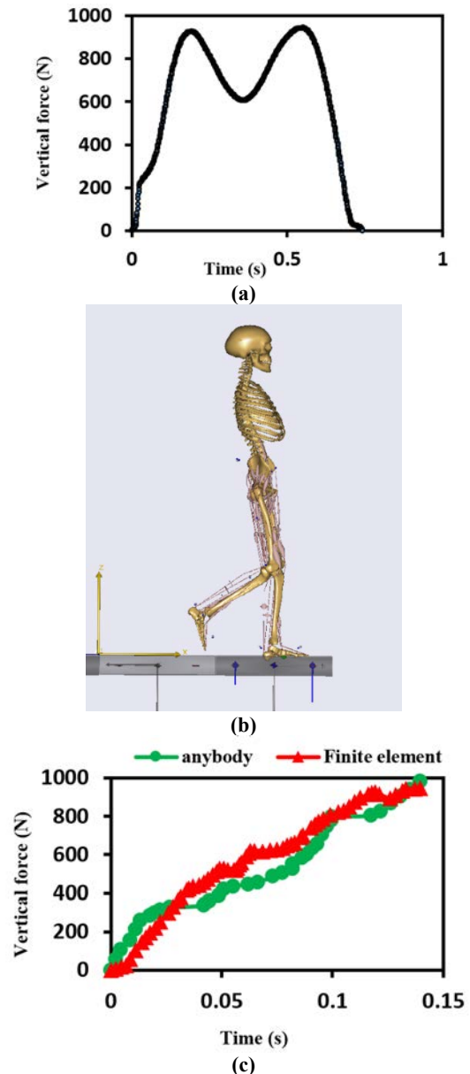
Figure 5 (a) Vertical force-time graph measured on the force plate for a barefoot male subject with a weight of 83 Kg. (b)
