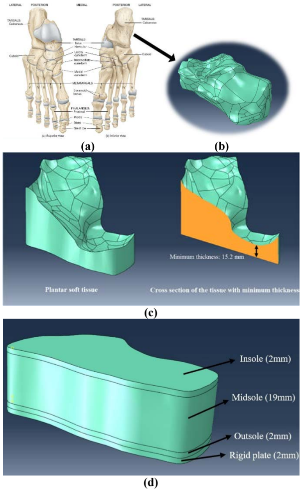
Figure 2 (a) Skeleton of the foot consists of tarsal bones, including talus and calcaneus [28]. (b) Imported calcaneus bone model in ABAQUS from point cloud provided by a CT-scan. (c) Plantar soft tissue under the calcaneus covered the lower surface of the calcaneus. (d) The sole
